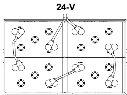
(4) 6-V BATTERY WIRING DIAGRAM
